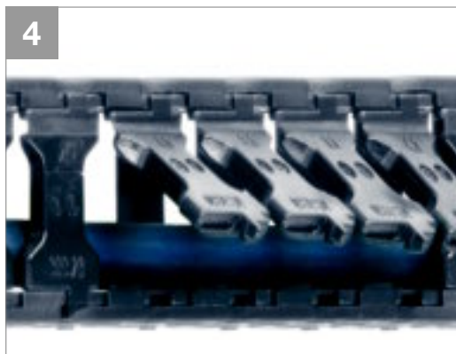
Speciality two-piece e-chains®: B07 and B09 snap-open along outer radius. Series 074 and 094 snap-open along inner radius
